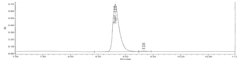
HPLC-UV Chromatogram
